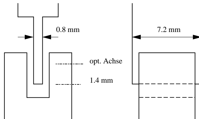
Figure 2. Mechanical setup
